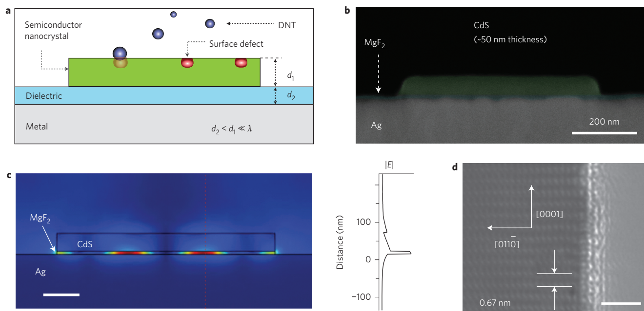
Figure 1 | Schematic, SEM image, simulated field distribution and transmission electron microscope (TEM) image of an active plasmon nanosensor.
